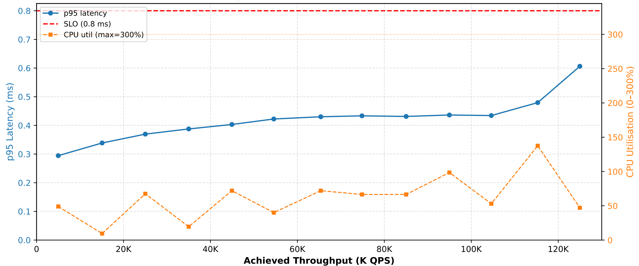
Q1d - T=3 threads, C=3 core(s)
