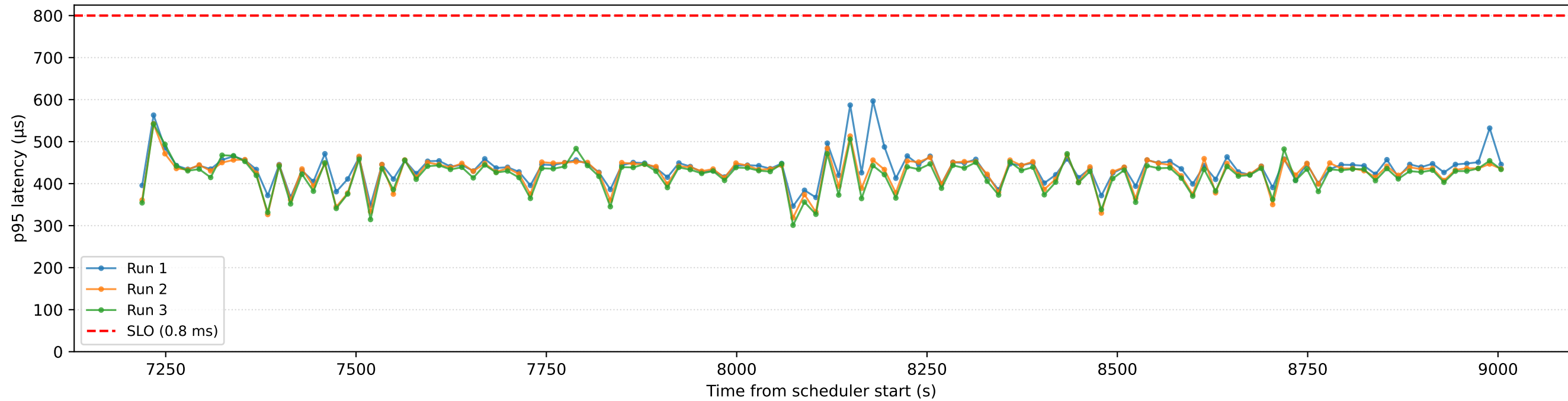
Part 4 — p95 latency across all 3 runs
