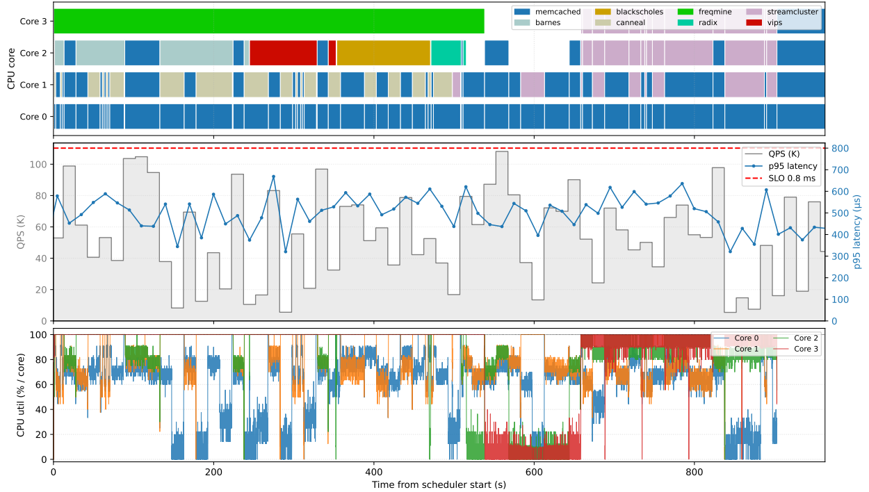
Figure 12: Part 4 Q3 Run 1, adaptive scheduler execution with interval=15 s. The controller achieves 0/56 SLO violations during the batch execution window, and 0/68 over the whole measurement trace. During the batch window, max p95 = 700.8 \mu s and mean p95 = 528.7 \mu s, remaining below the 0.8 ms threshold. The batch makespan is 838.4 s, and peak CPU utilization reaches 100% on all four cores during the heaviest phases, showing that the scheduler keeps the machine saturated while preserving memcached latency within the SLO.
