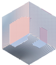
Geometry Recon.
