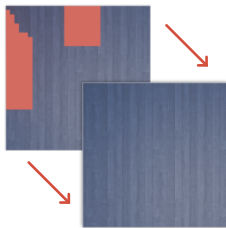
Texture Inpainting
