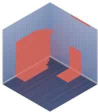
Mesh Creation
