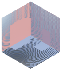
Plane Refinement
