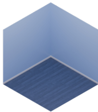
Scene Completion
