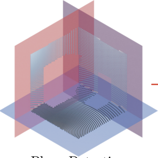
Plane Detection
