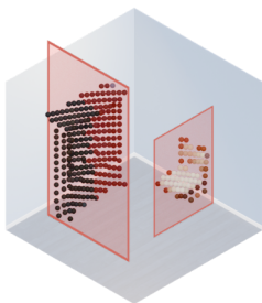
Symmetry Detection
