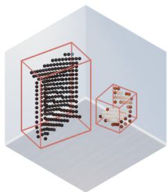
Object Detection
