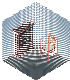
Refined Objects
