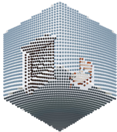
Aligned Pointcloud
