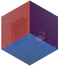
Plane Segmentation
