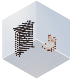
Structural Removal
