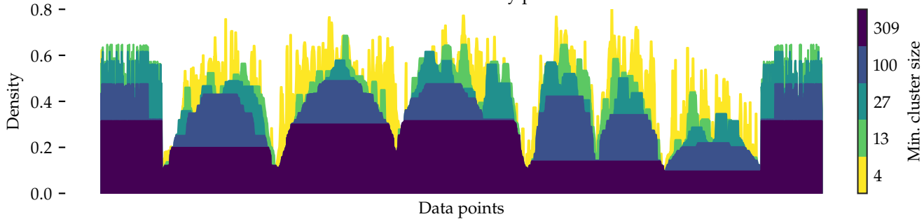
HDBSCAN* density profile
