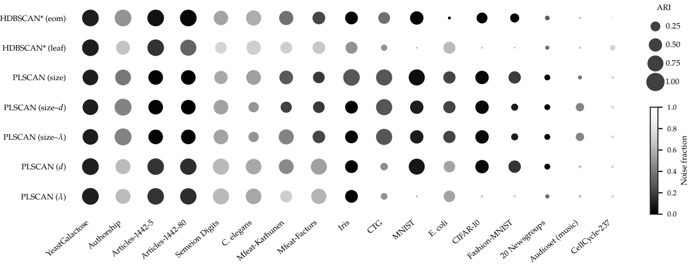
ARI (size) and noise fraction (shade) at k = 4
