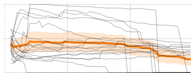
HDBSCAN* (leaf)
