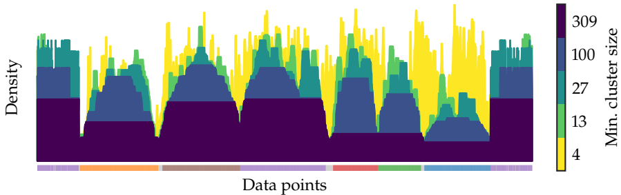
HDBSCAN* density profile
