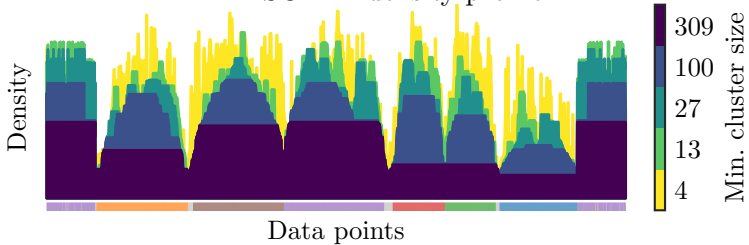
HDBSCAN* density profile
