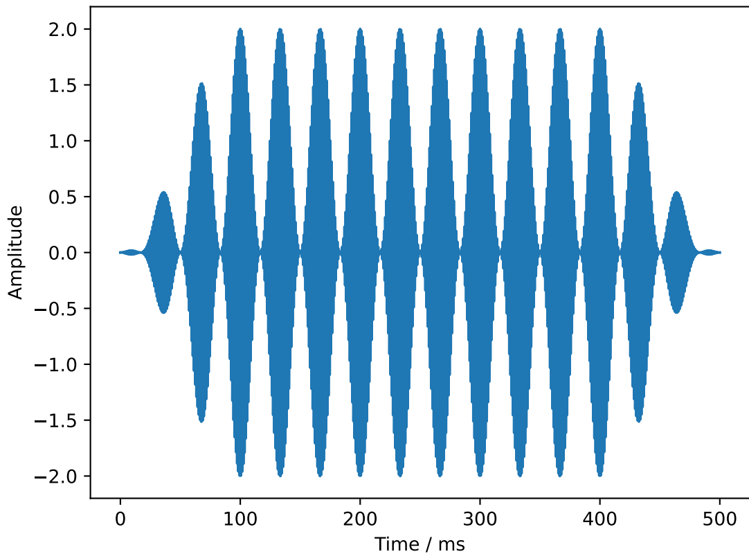
1kHz tone with 30Hz modulator
