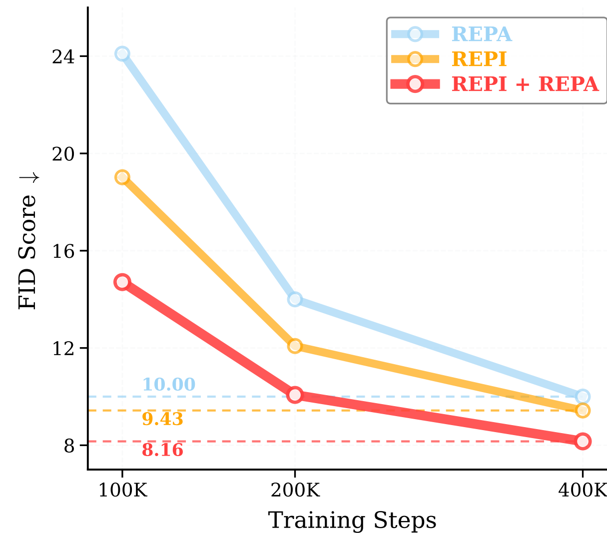
SiT-L/2
