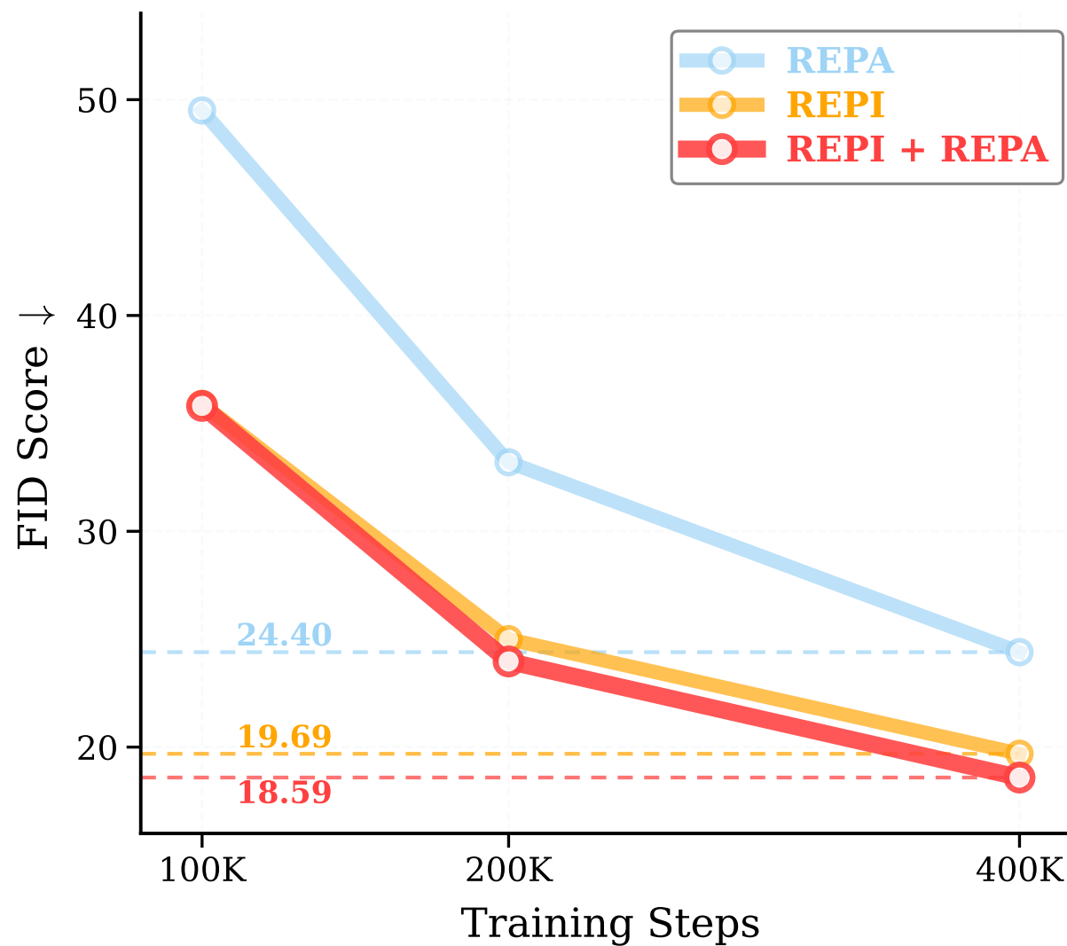
SiT-B/2
