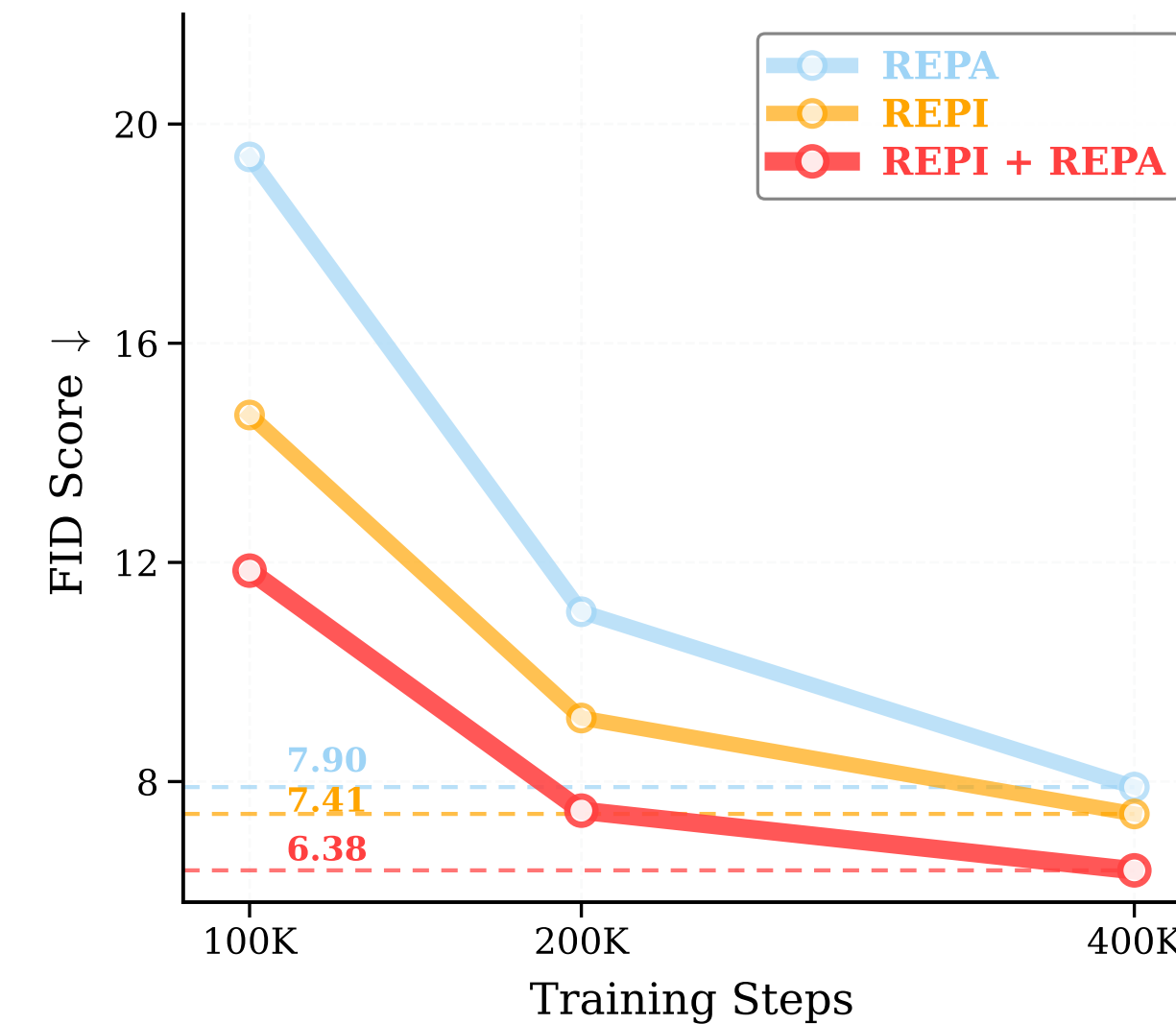
SiT-XL/2
