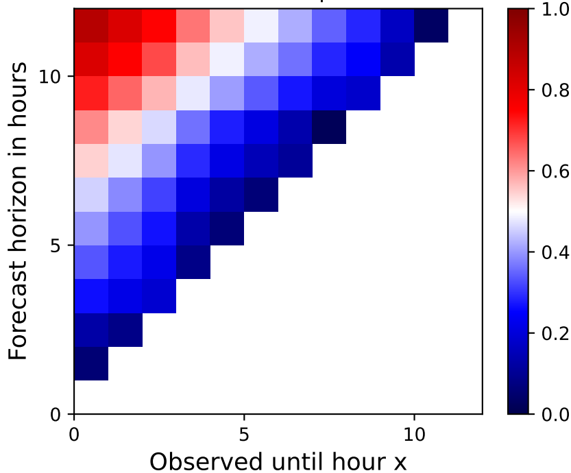
ALT Root Mean Square Error
