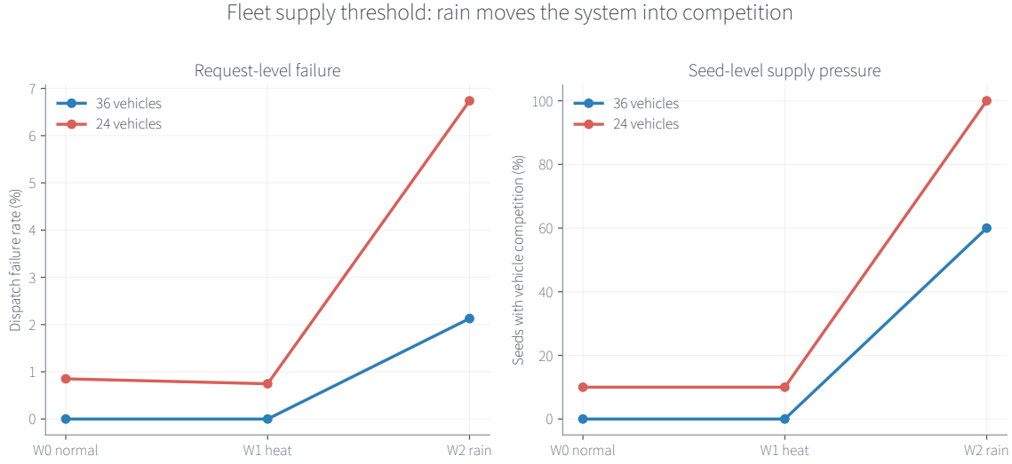
Figure 11: Request failure and share of competing seeds with 36 versus 24 vehicles.
