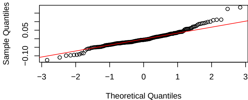
Q-Q Plot of Residuals
