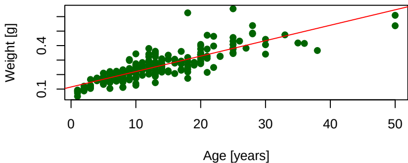
Scatter Plot with Linear Fit
