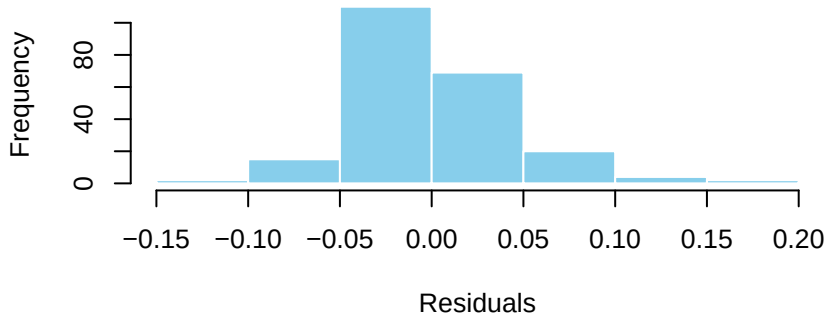
Histogram of Residuals
