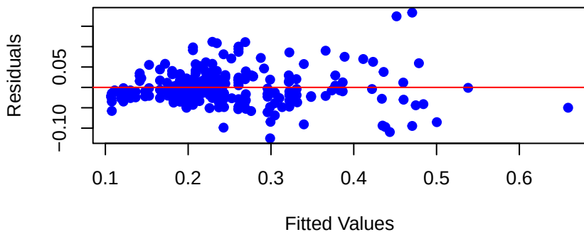
Residuals vs Fitted Values
