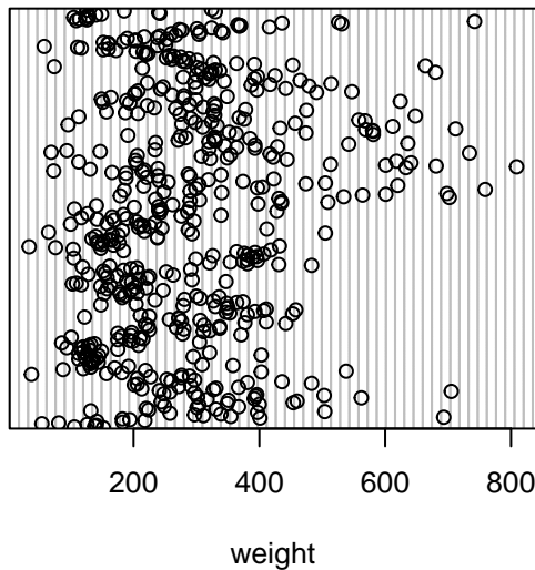
Dotchart: weight
