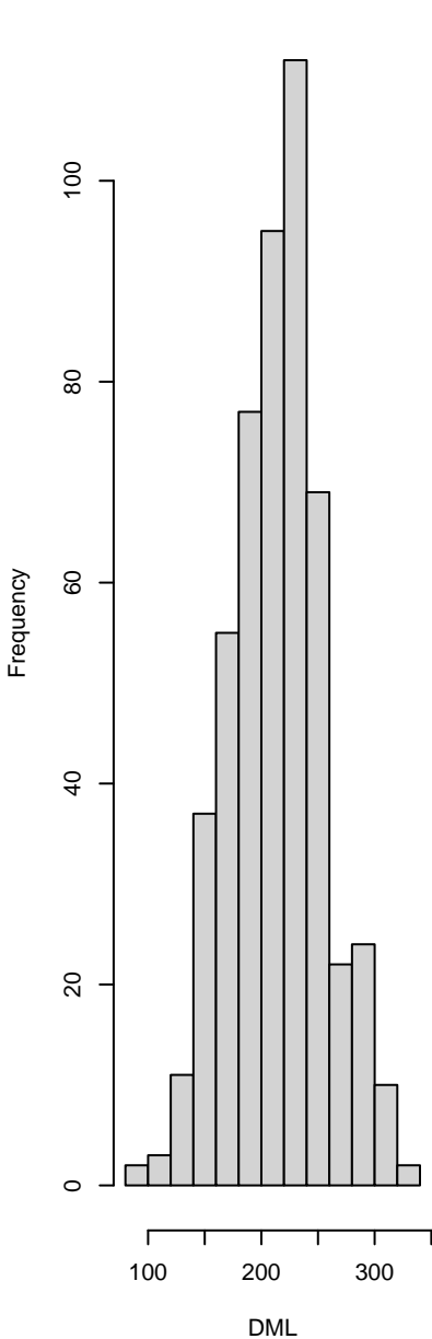
DML (breaks=10)
