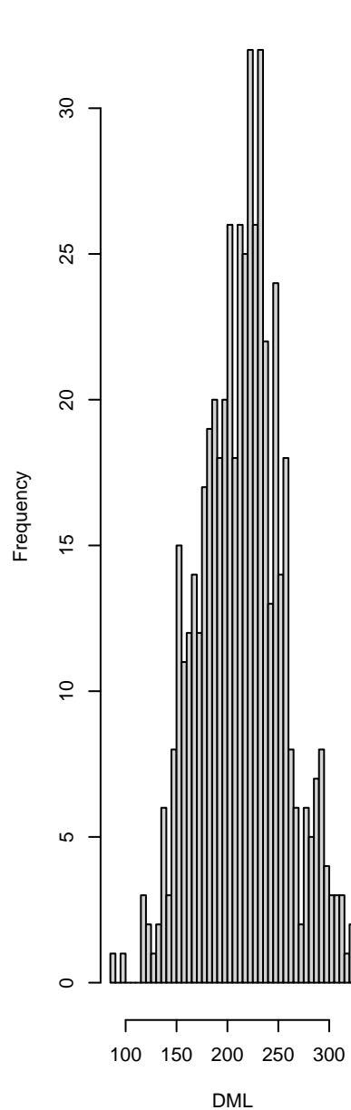
DML (breaks=40)
