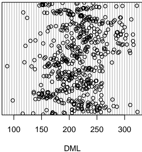
Dotchart: DML
