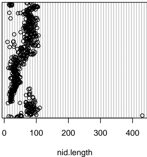
Dotchart: nid.length
