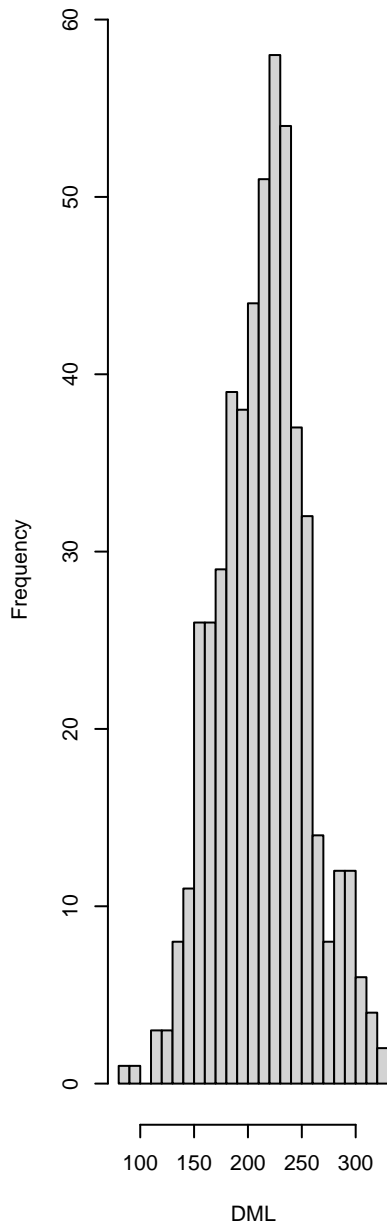
DML (breaks=20)
