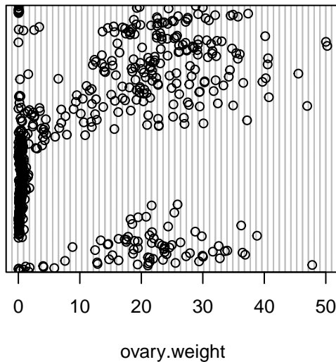
Dotchart: ovary.weight
