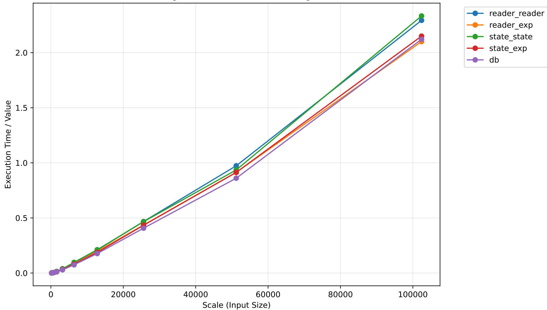
VC generation with Let and Assign
