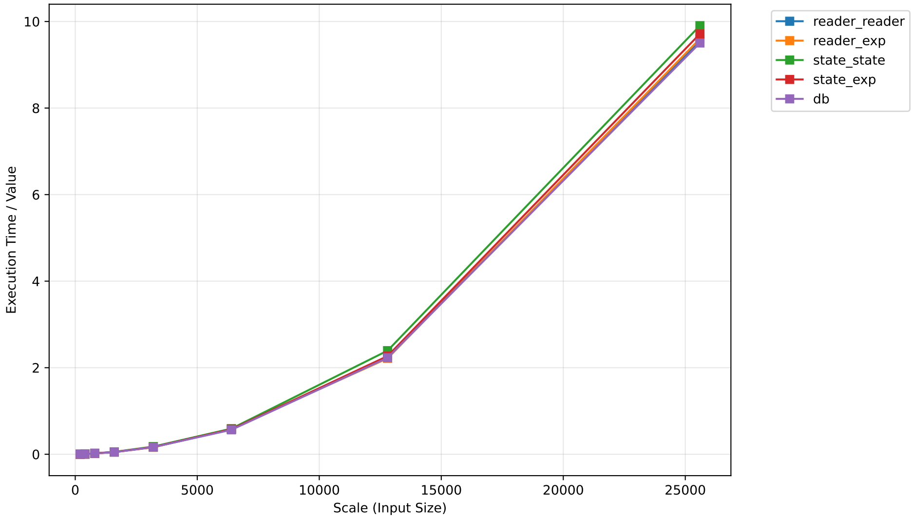
VC generation with Recursion (Linear Scale)
