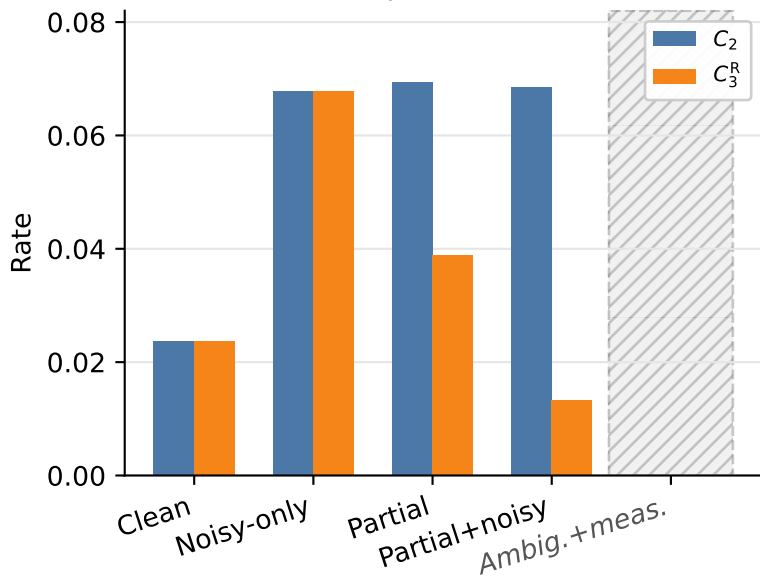
(a) False-safe fidelity rate
