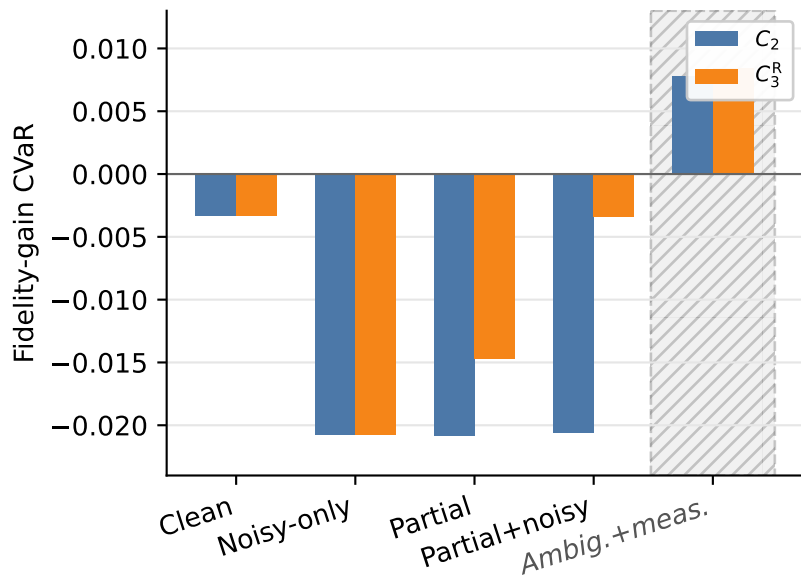
(b) Lower-tail CVaR 0.05
