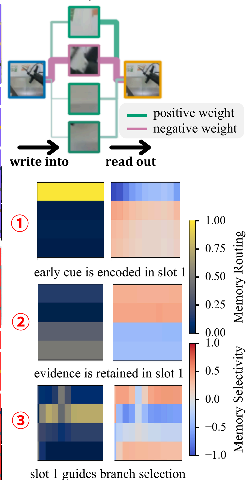
memory slots
