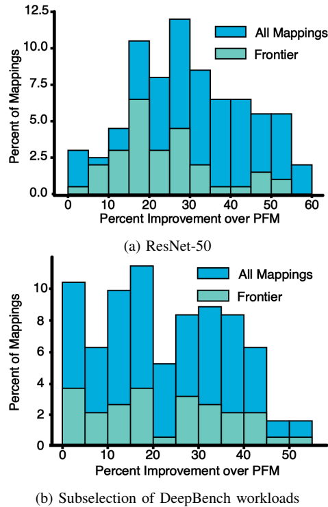
Fig. 14: Evaluating different PE configurations for an Eyeriss-like architecture ( 2 \times 7 to 16 \times 16 ) for ResNet-50 (a) and DeepBench (b). Ruby-S improves performance while forming a new Pareto frontier.
