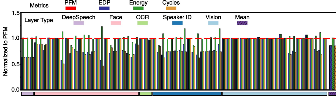
Fig. 11: Comparison between mappings generated by Ruby-S, normalized to PFM over a selection of workloads from DeepBench optimized for EDP [37].
