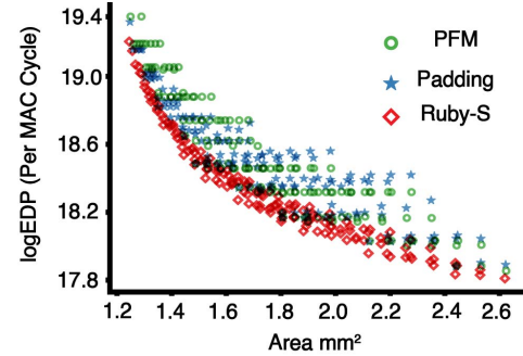
(a) ResNet-50
