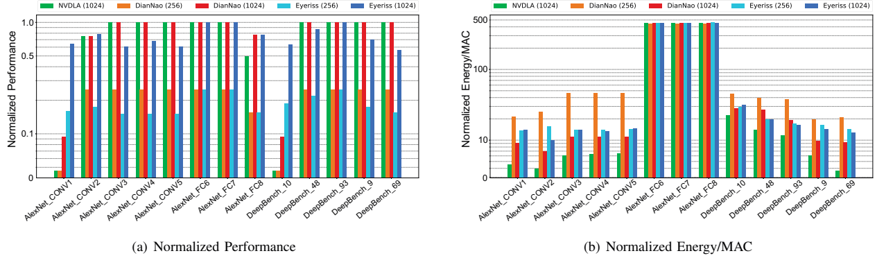
Fig. 14. Performance and Energy Efficiency Comparisons of NVDLA, DianNao, and Eyeriss.
