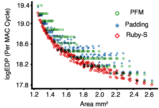
(a) ResNet-50
