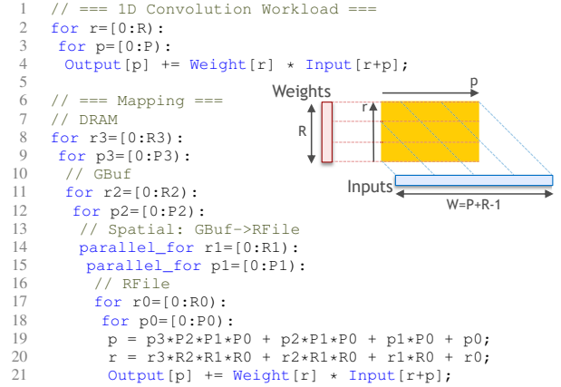
Fig. 5. Example mapping of a 1D convolution onto the Eyeriss organization. Inset: the projections defined by this workload from the operation space to the input and weight dataspace.
