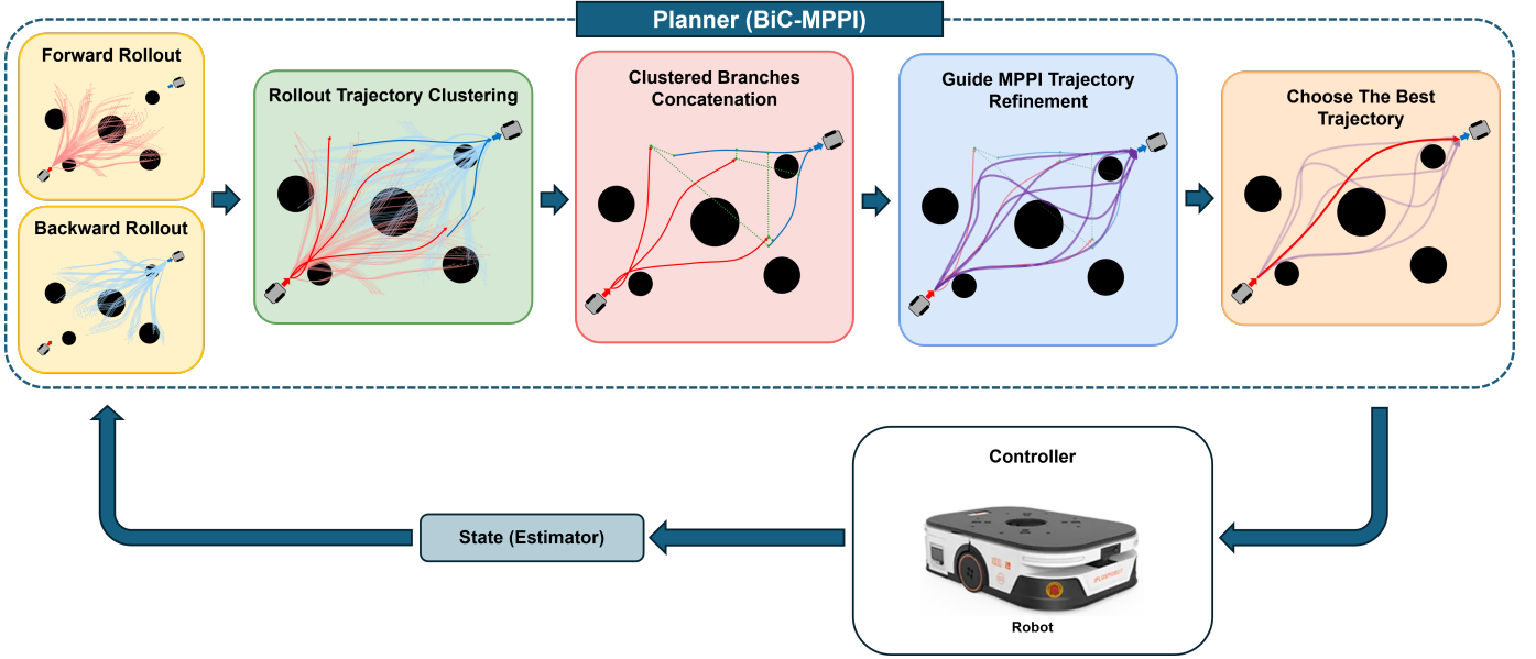
Fig. 1. Overview of the proposed BiC-MPPI framework. The final panel selects the lowest-cost refined candidate and applies its first control in receding-horizon form.
