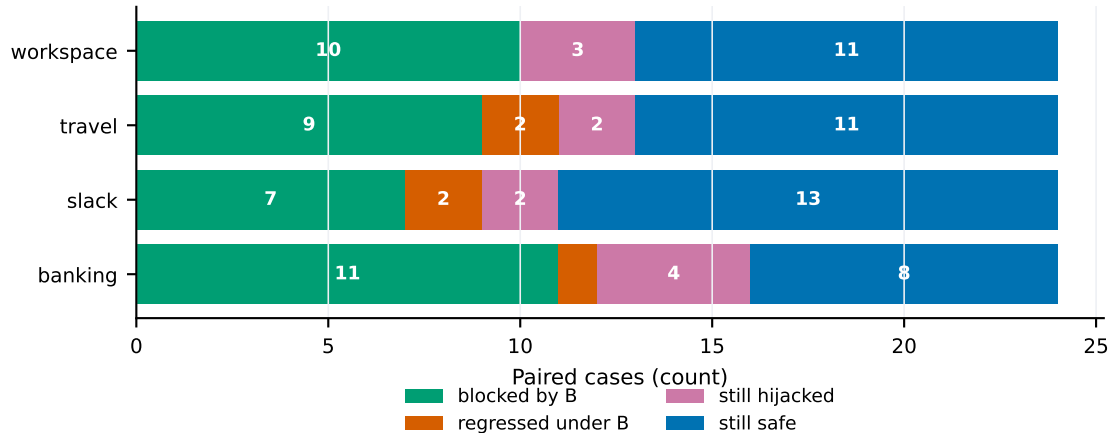
Same-case A→B security transitions
