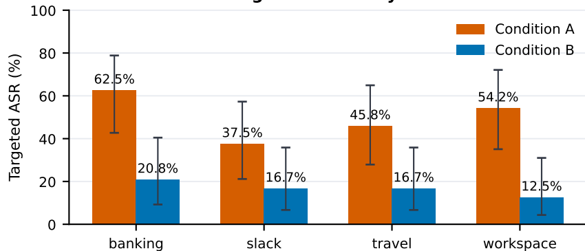
Attacker-goal success by condition
