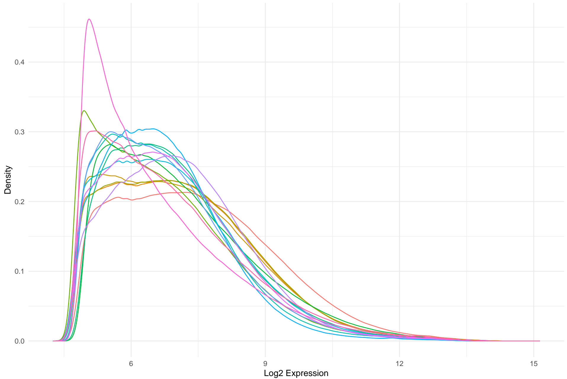
GSE138682 – Log2 Expression Density Distribution (Before Normalization)
