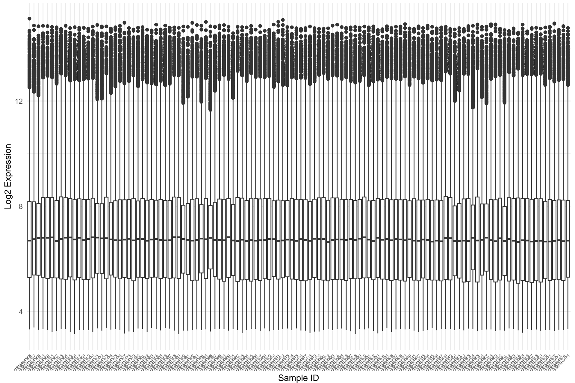
GSE19804 – Log2 Expression Distribution (After Normalization)
