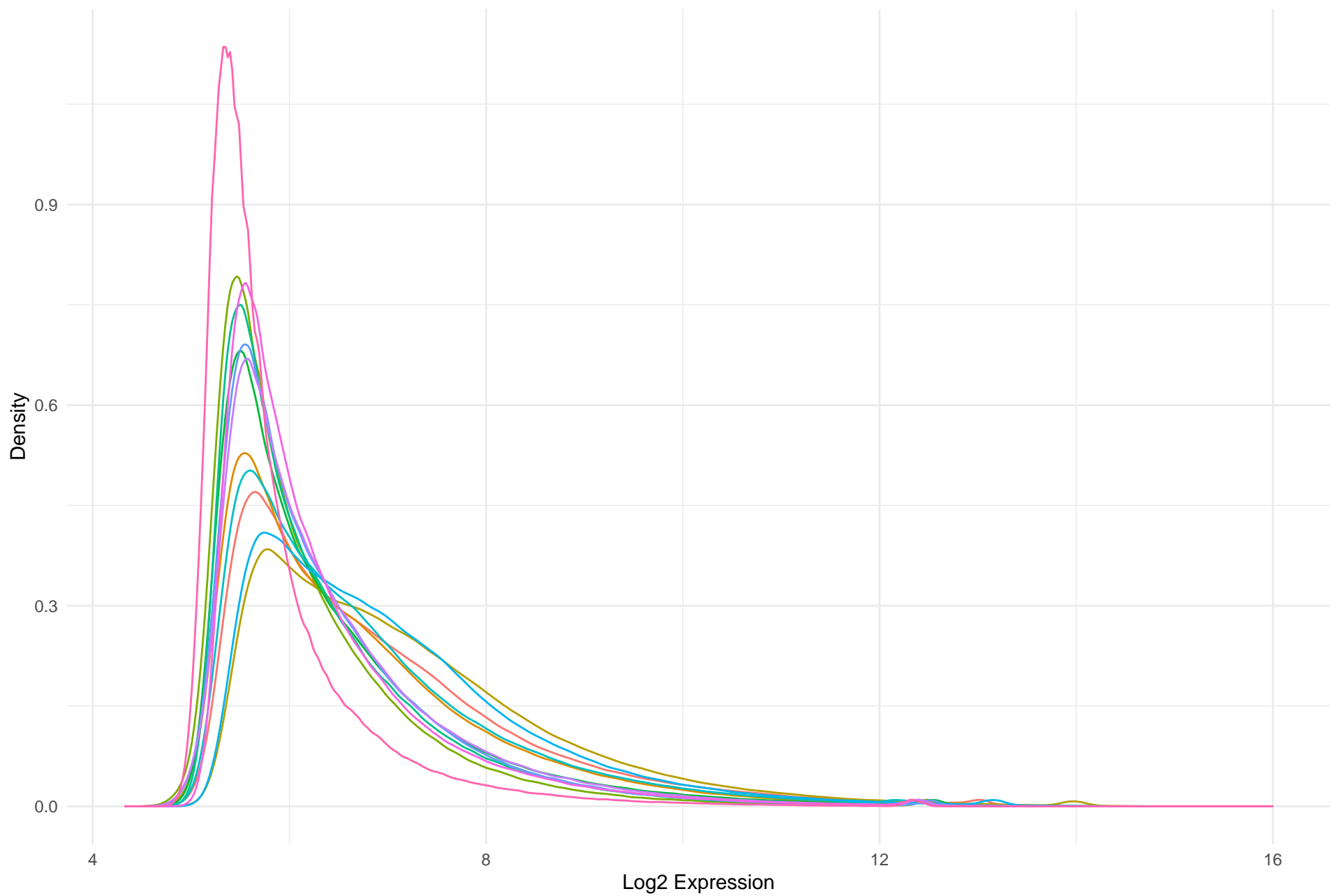
GSE118370 – Log2 Expression Density Distribution (Before Normalization)
