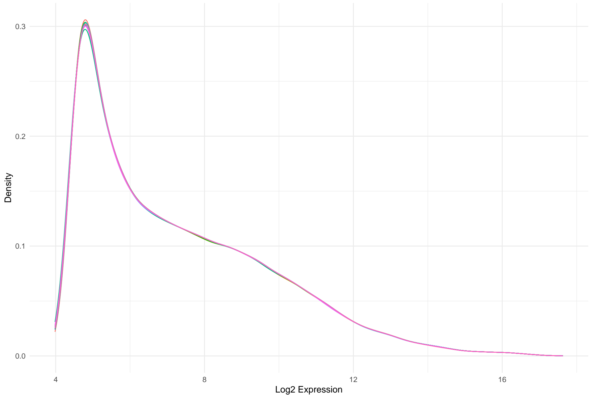
GSE136043 – Log2 Expression Density Distribution (After Normalization)
