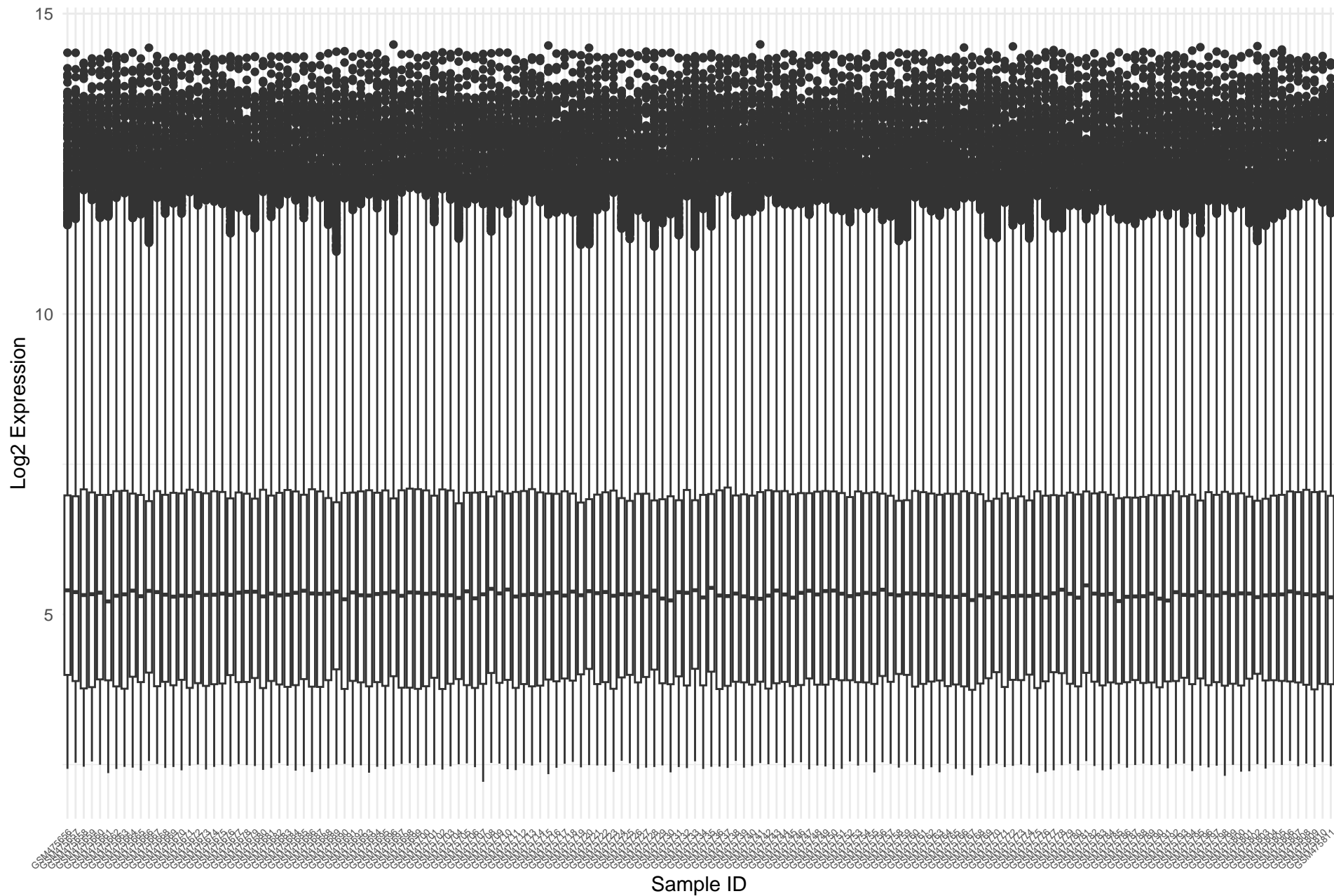
GSE19188 – Log2 Expression Distribution (After Normalization)
