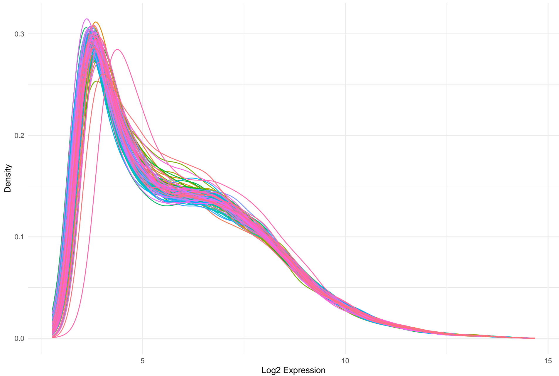
GSE18842 – Log2 Expression Density Distribution (After Normalization)
