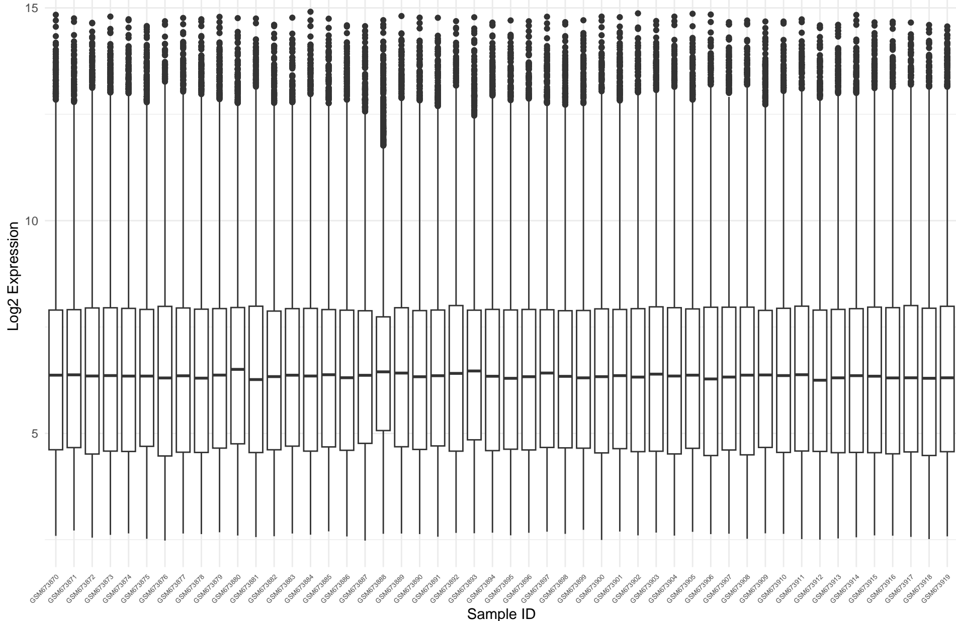
GSE27262 – Log2 Expression Distribution (After Normalization)
