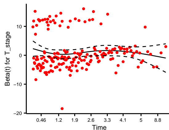
Schoenfeld Individual Test p: 0.0467
