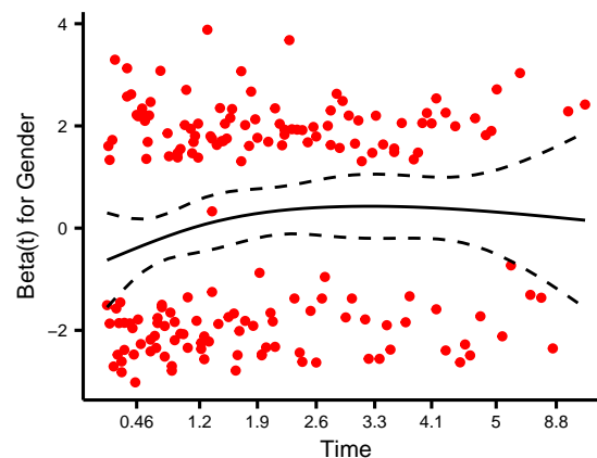
Schoenfeld Individual Test p: 0.8739
