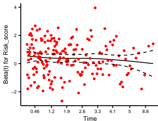
Schoenfeld Individual Test p: 0.0293
