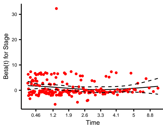
Schoenfeld Individual Test p: 0.312
