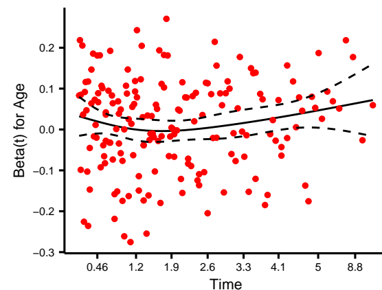
Schoenfeld Individual Test p: 0.1861
