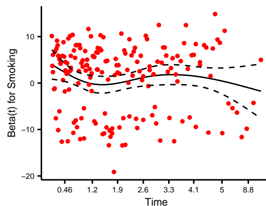
Schoenfeld Individual Test p: 0.0467
