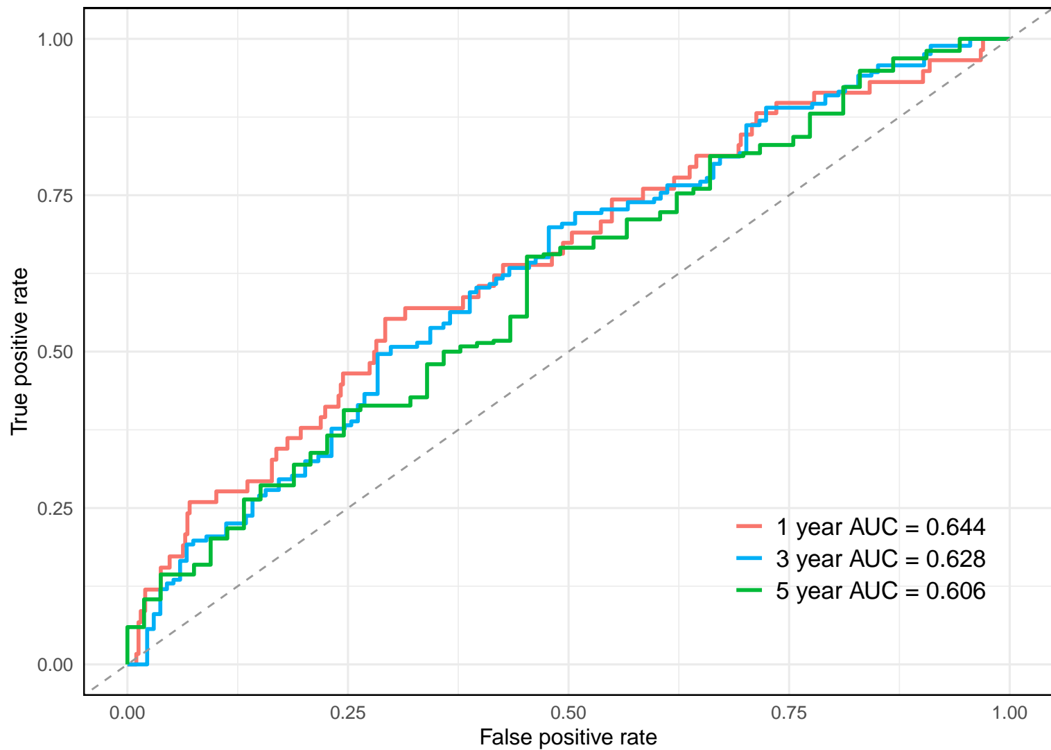
ROC curves
