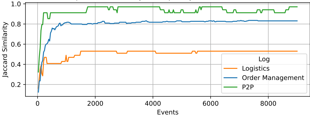
Jaccard Similarity - (Frequency Threshold: 0.05)
