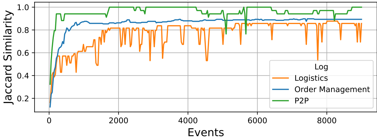
Jaccard Similarity - (Window Size: 125)
