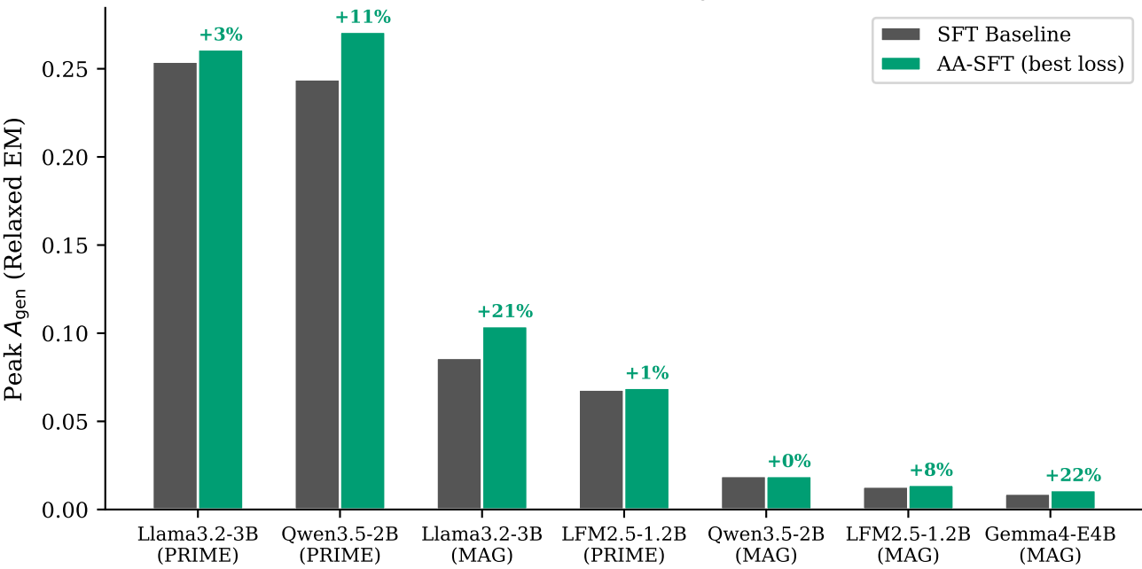
AA-SFT vs. SFT Baseline — Peak A_{\text{gen}} (6/7 pairs improved)
