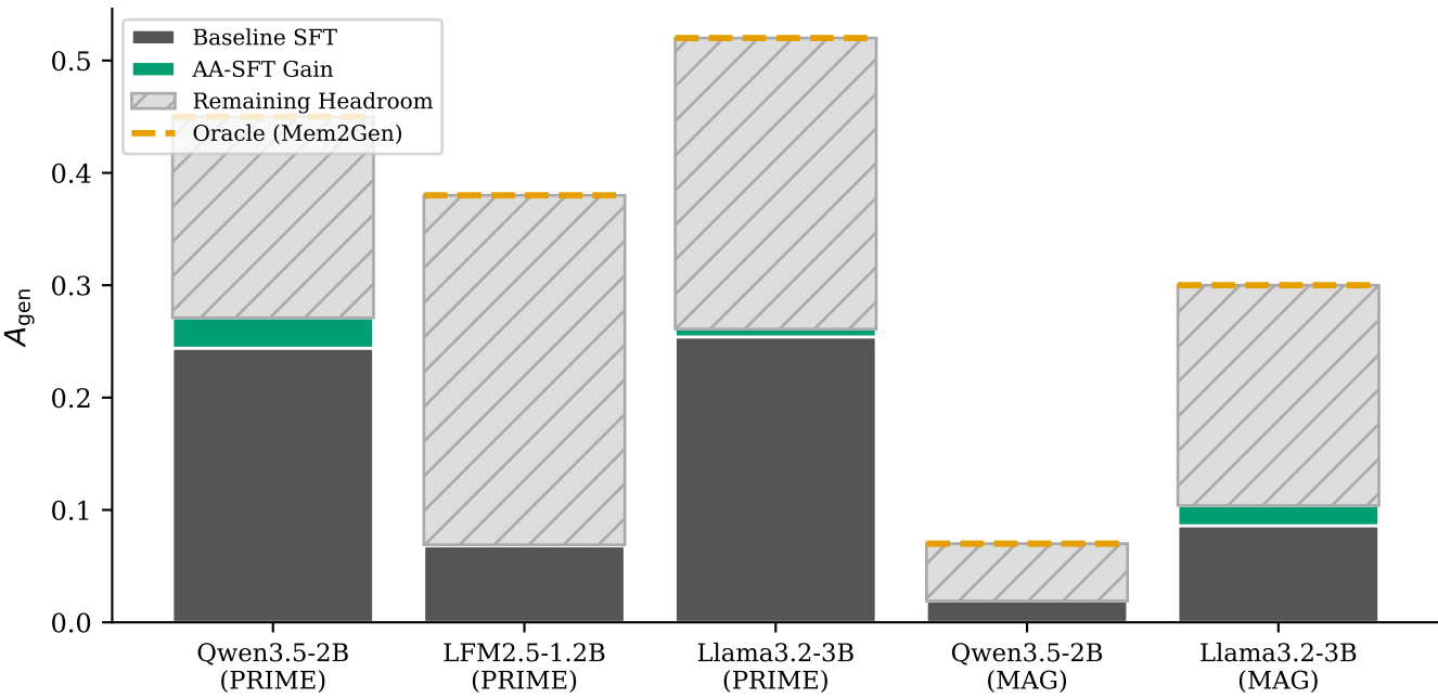
Oracle Headroom: Fraction of Gap Closed by AA-SFT (Relaxed EM)
