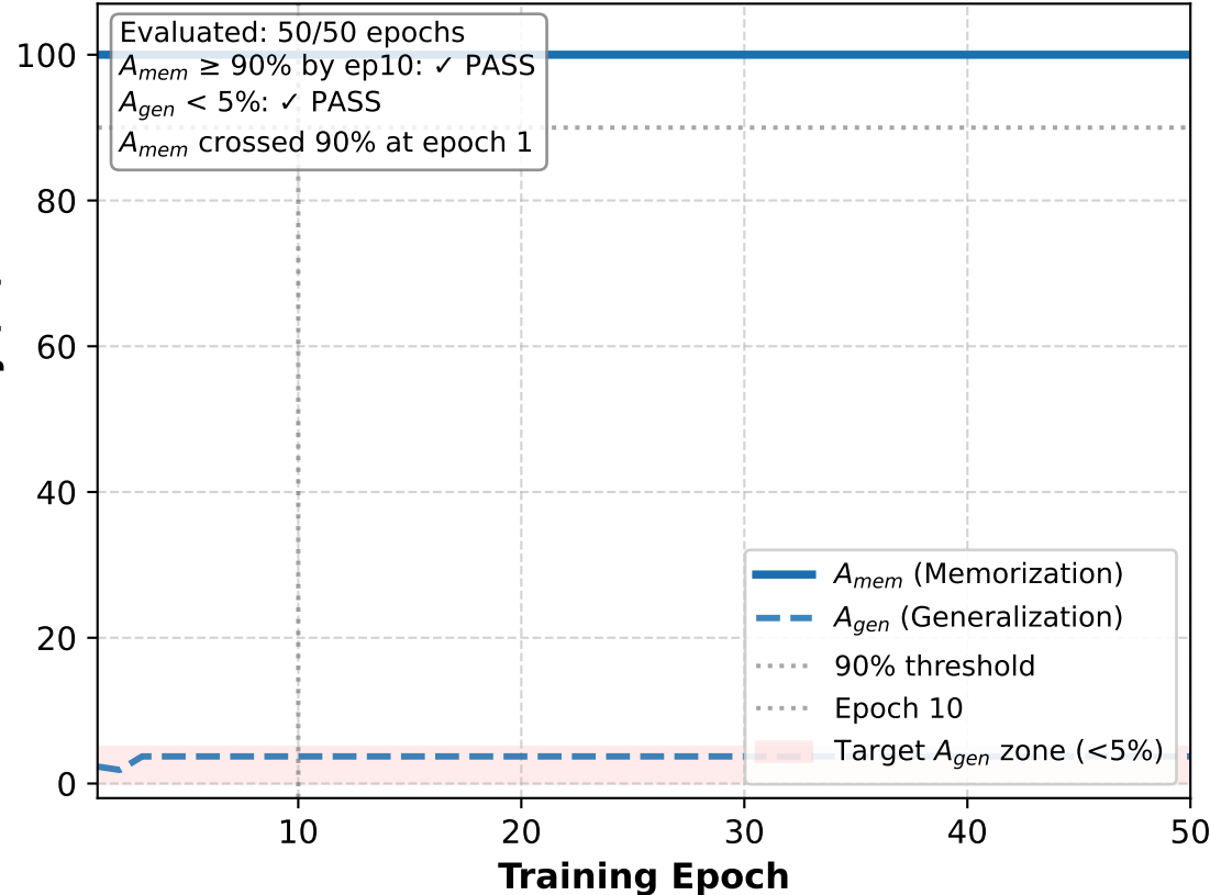
Task A: Chaining (Multi-hop Reasoning)
