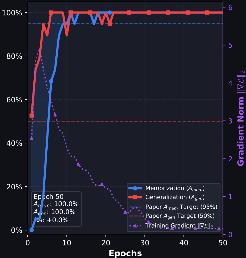
Task C: Fact Checking
