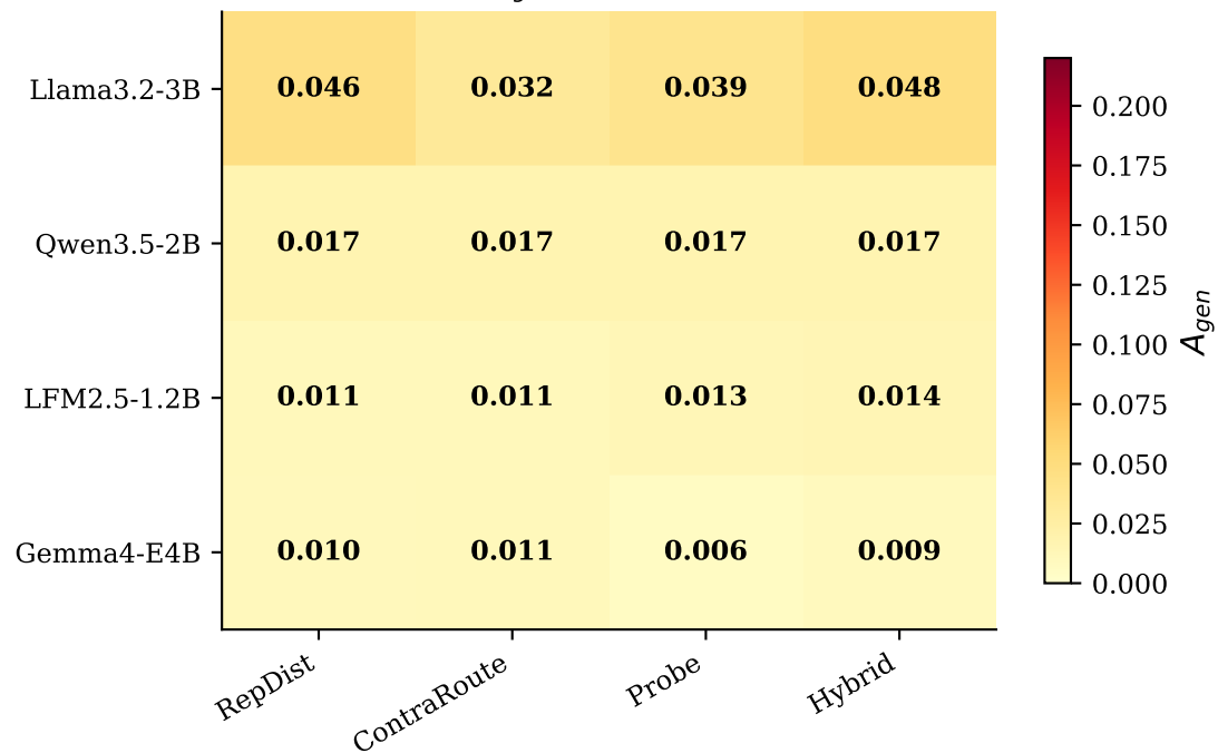
Peak A_{gen} — STaRK-MAG
