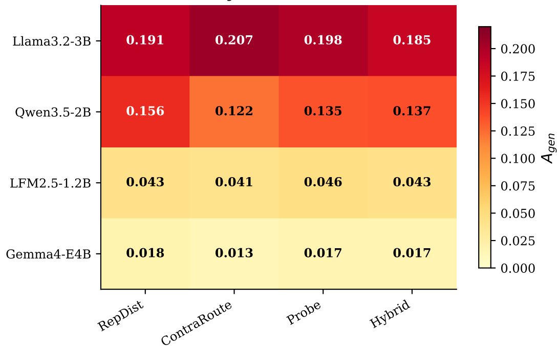
Peak A_{gen} — STaRK-PRIME
