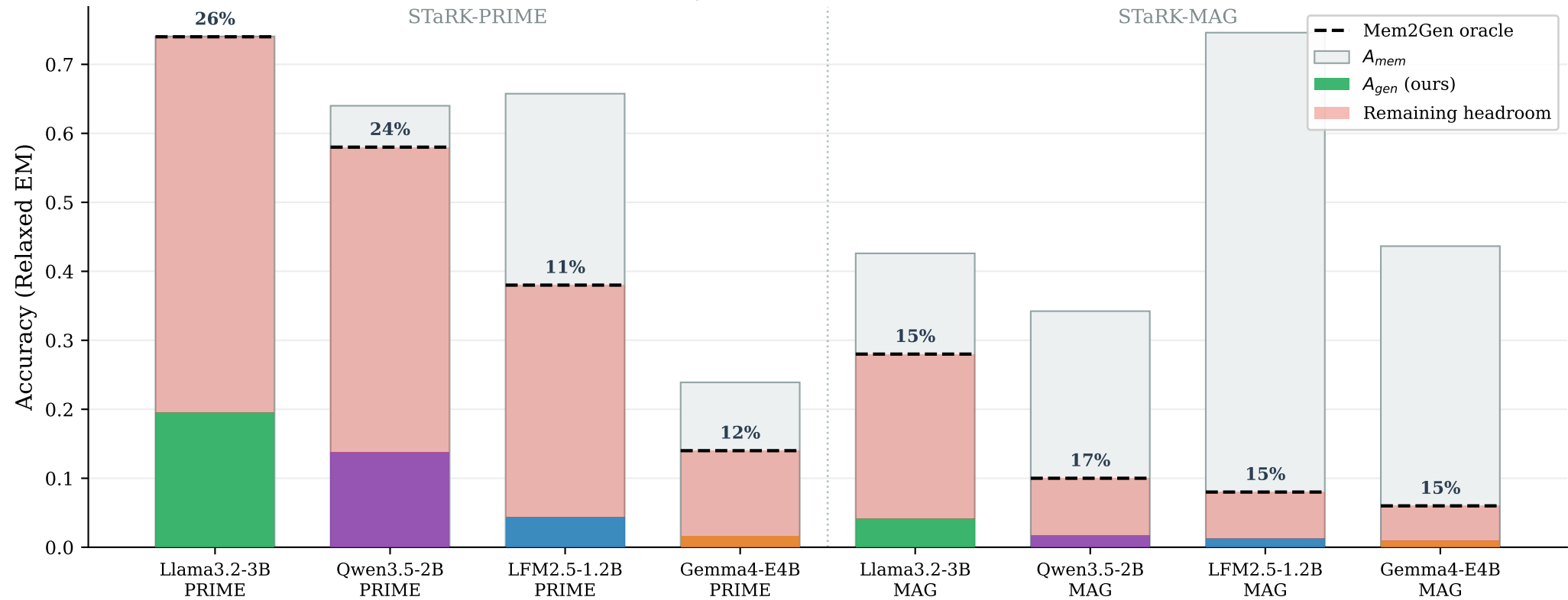
Oracle Headroom Analysis % = A_{gen} fraction of oracle gap closed
