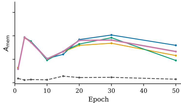
Qwen3.5-2B / STaRK-MAG
