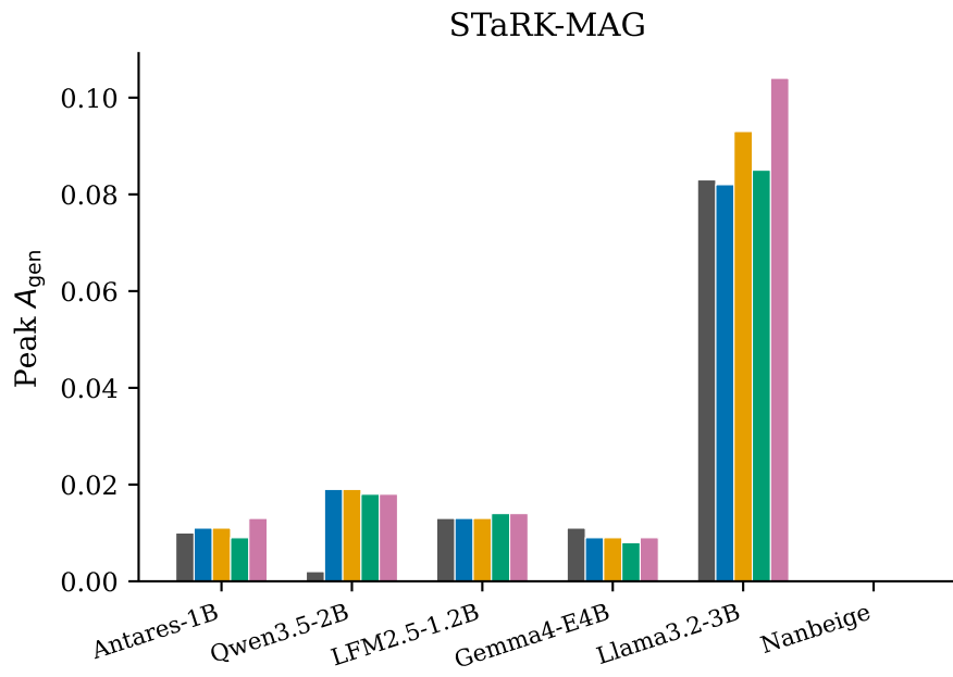
V1 Alignment Loss Variants vs. Baseline SFT — Peak A_{\text{gen}}
