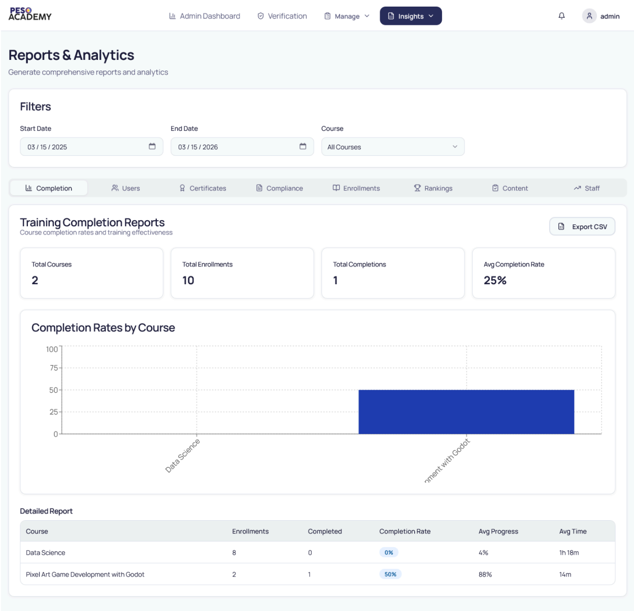
Figure 9: Admin - Reports
