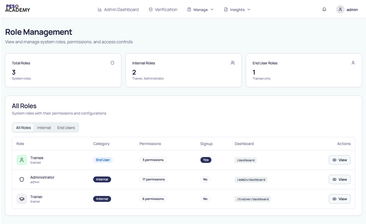
Figure 3.2: Admin - Role Management
