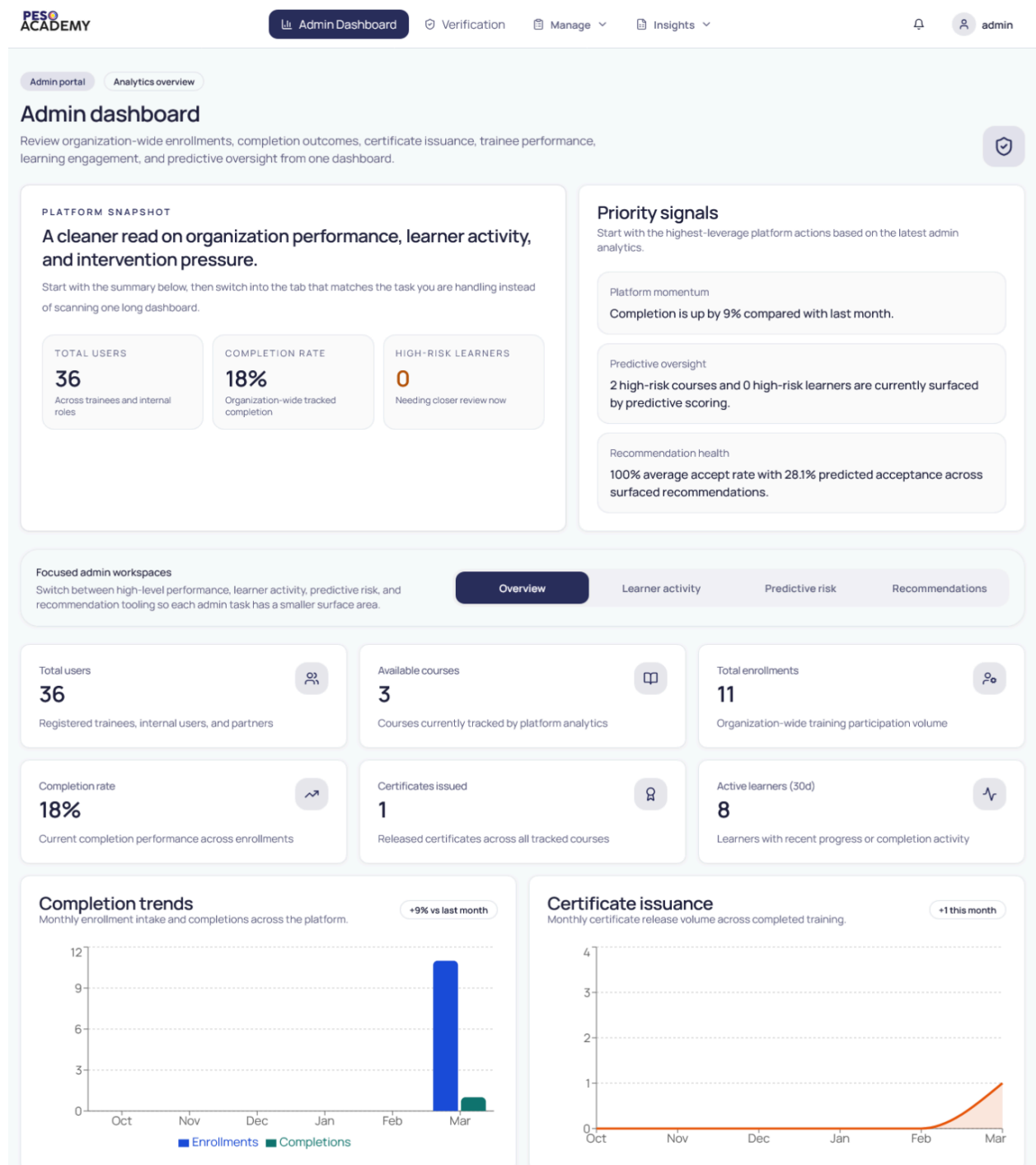
Figure 1: Admin Dashboard
