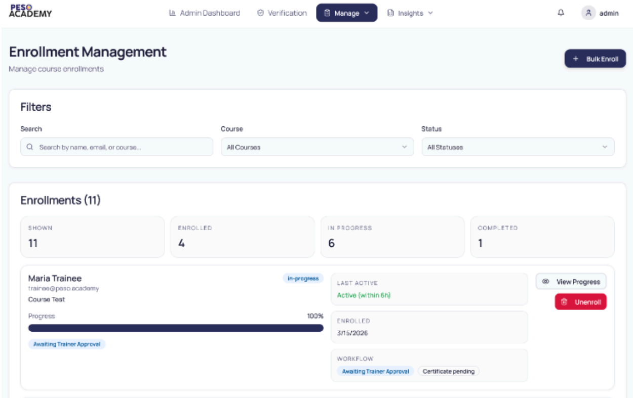
Figure 7: Admin - Enrollment Management
