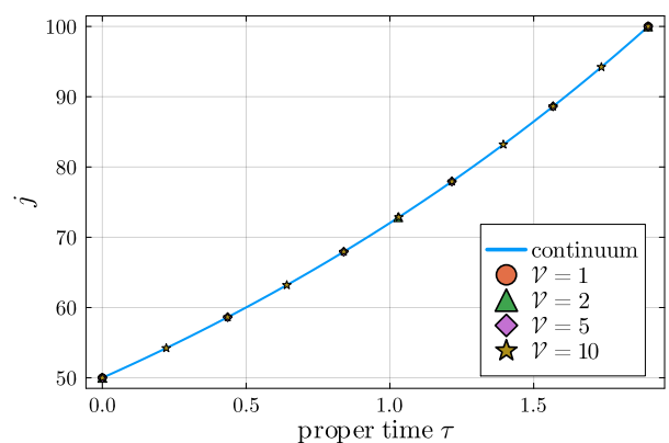
FIG. 6: Continuum and discrete area of spacelike slices as a function of proper time \tau with (\mathcal{V}_T, \mathcal{V}_S) = (\mathcal{V}, \kappa_* \mathcal{V}) . Evidently, increasing \mathcal{V} only leads to a finer sampling of the continuum solution. The boundary data and \Lambda have been fixed to j_0 = 50 , j_{\mathcal{V}_T} = 100 , and \Lambda = 0.1 .
