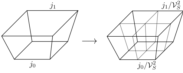
FIG. 3: Refinement of frustum geometry with total areas j_0 and j_1 . Individual frusta are rescaled as (j_0, j_1) \rightarrow (j_0/V_S^2, j_1/V_S^2) . For illustrative purposes, one spatial dimension is suppressed.
