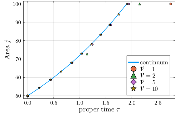
FIG. 5: Continuum and discrete area of spacelike slices as a function of proper time \tau . The boundary data and \Lambda have been fixed to j_0 = 50 , j_{V_T} = 100 , and \Lambda = 0.1 .
