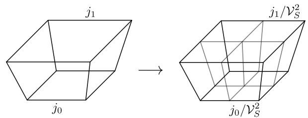
FIG. 3: Refinement of frustum geometry with total initial square area j_0 and final square area j_1 . Individual frusta are rescaled as (j_0, j_1) \rightarrow (j_0/\mathcal{V}_S^2, j_1/\mathcal{V}_S^2) . For illustrative purposes, one spatial dimension is suppressed.
