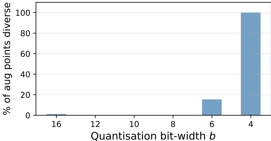
CNN — diverse aug points per b
