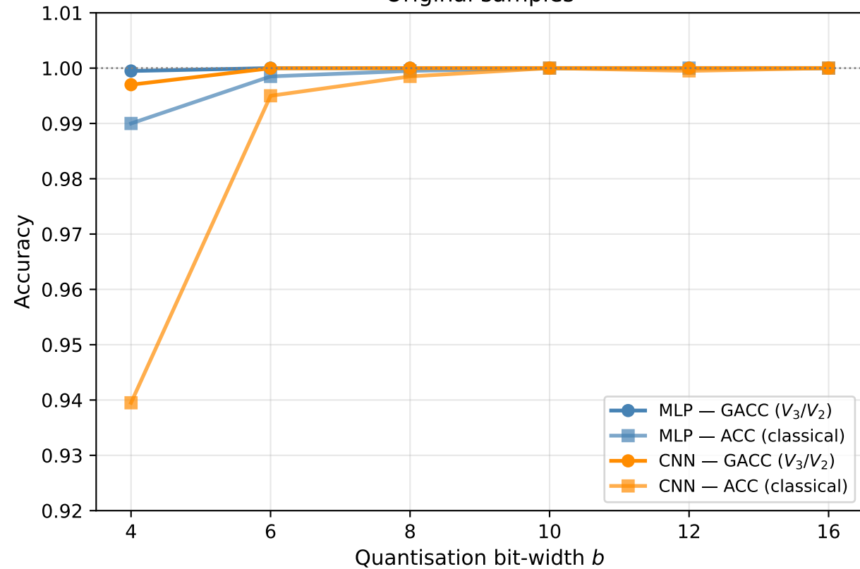
Original samples
