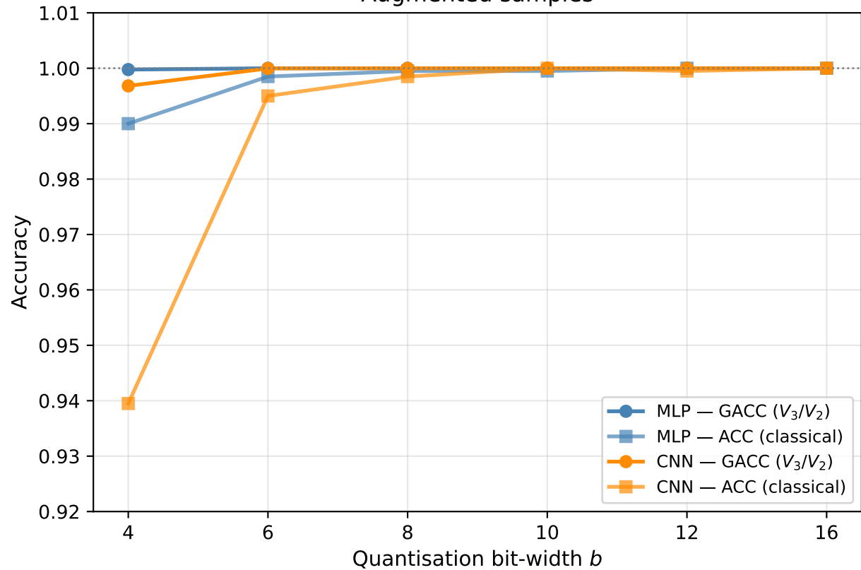
Augmented samples
