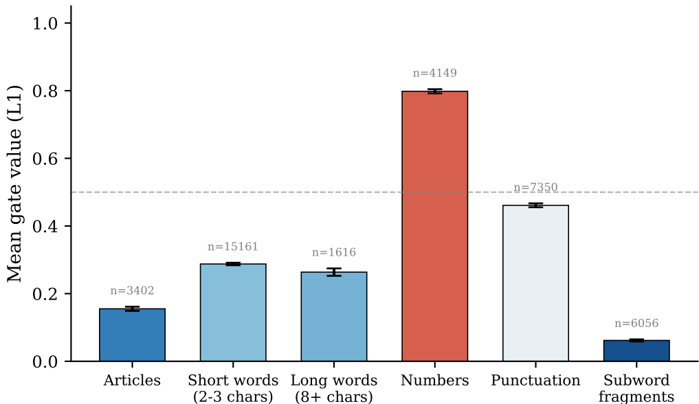
Gate Value by Token Category (Layer 1)
