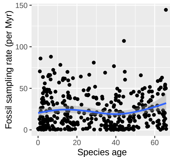
Predictor: age
