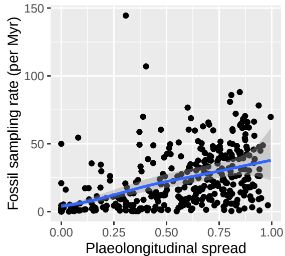
Predictor: plaeolong. spread
