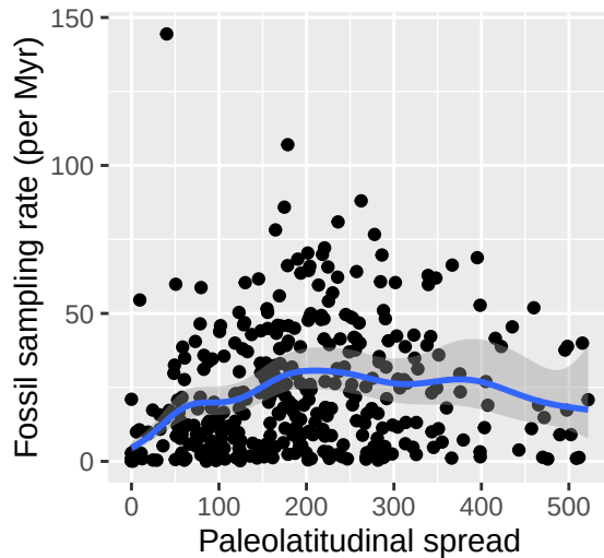
Predictor: paleolat. spread
