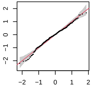
deviance residuals
