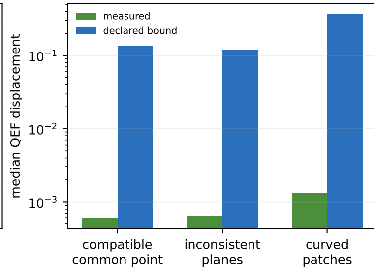
(c) Bound conservatism
