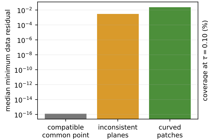
(a) Compatibility of true planes
