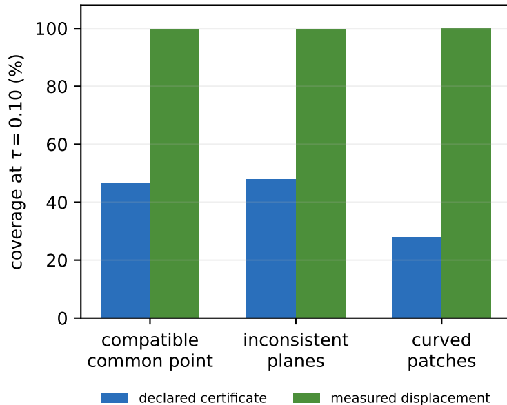
(b) Soundness versus usefulness
