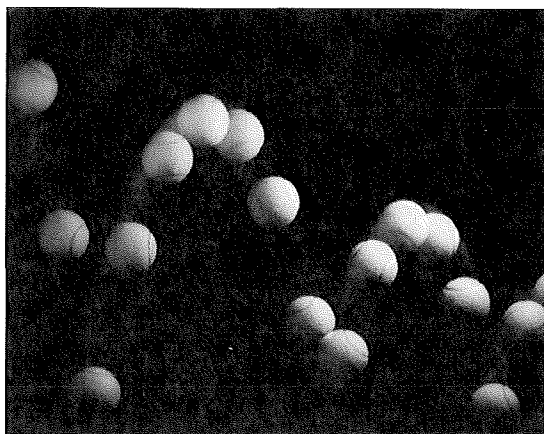
Fig. 4-8 A stroboscopic photograph of a yellow tennis ball bouncing off a hard surface. Between impacts, the ball has projectile motion. Source: Richard Megna/Fundamental Photographs.
