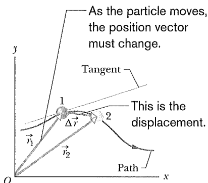
Fig. 4-3 The displacement \Delta\vec{r} of a particle during a time interval \Delta t , from position 1 with position vector \vec{r}_1 at time t_1 to position 2 with position vector \vec{r}_2 at time t_2 . The tangent to the particle's path at position 1 is shown.
