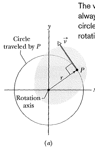
Fig. 10-9 The rotating rigid body of Fig. 10-2, shown in cross section viewed from above. Every point of the body (such as P ) moves in a circle around the rotation axis. (a) The linear velocity \vec{v} of every point is tangent to the circle in which the point moves. (b) The linear acceleration \vec{a} of the point has (in general) two components: tangential a_t and radial a_r .
